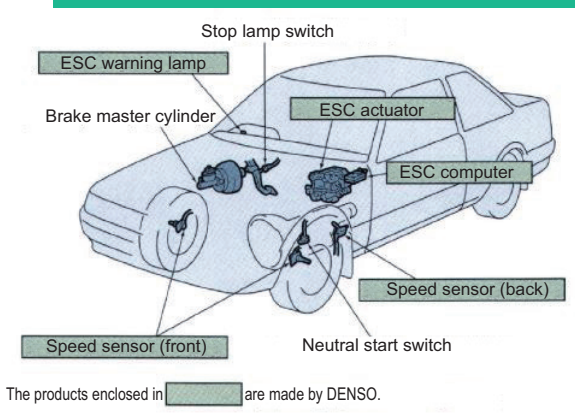
ABS in-vehicle system diagram
